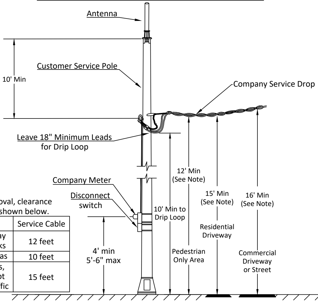
DIAGRAM "A" - CUSTOMER SERVICE POLE DETAILS (SIDE VIEW)
