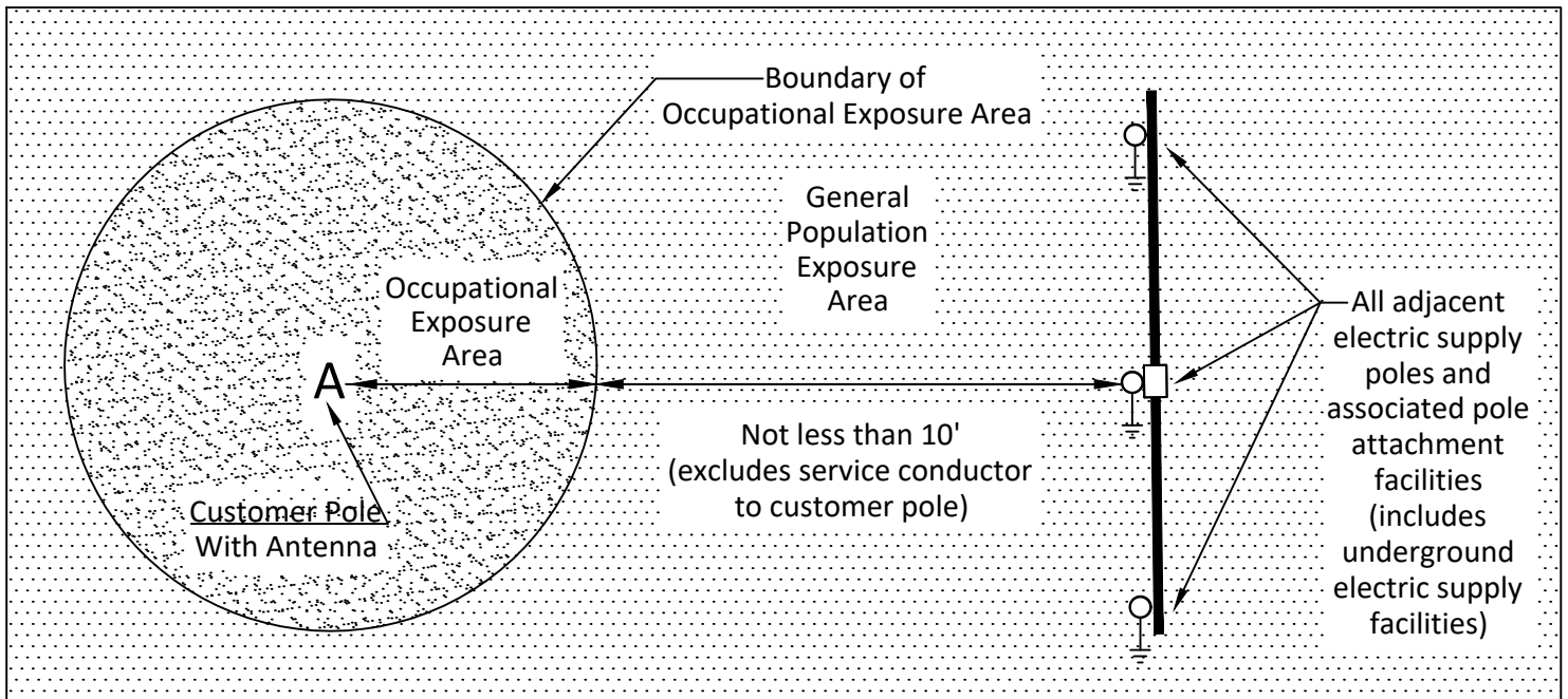
DIAGRAM "B" - RADIO FREQUENCY EXPOSURE AREA (TOP VIEW)
